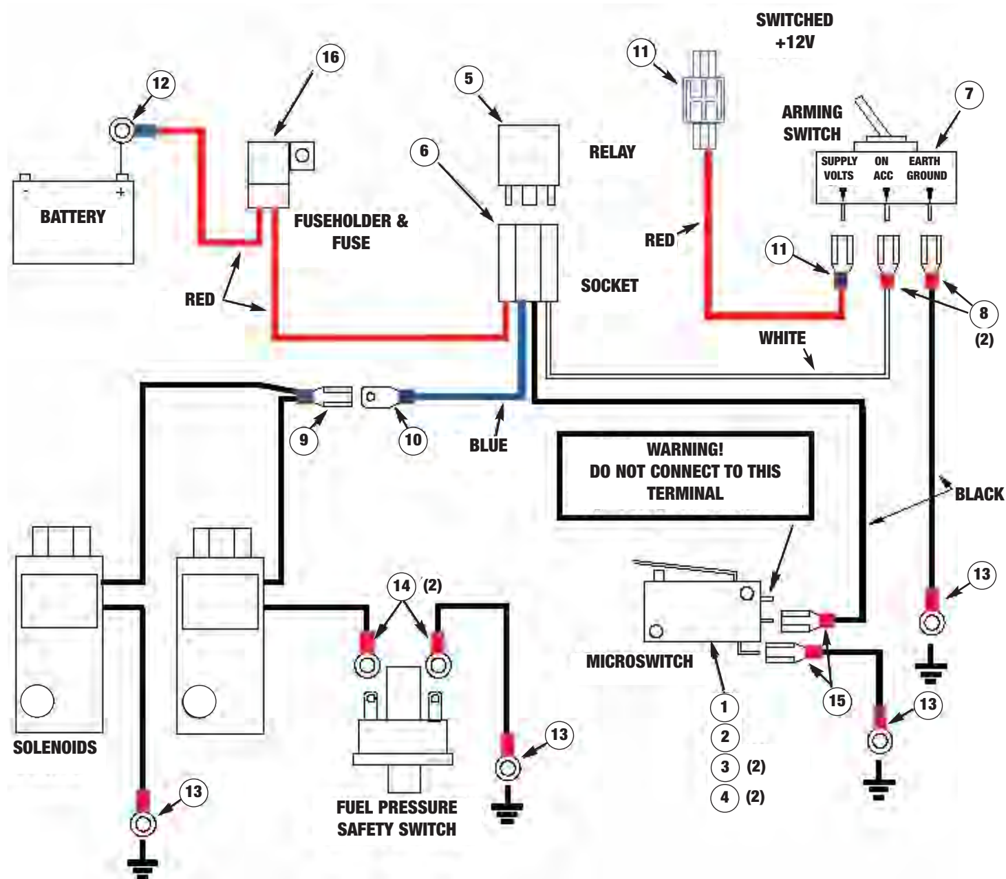
Wire Schematic Origin and Destination Map
