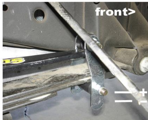
install hardware clear of factory sensor at axle rear
