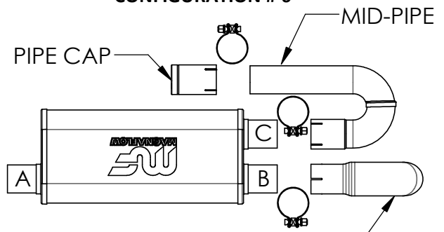
CLAMP-ON TIP
