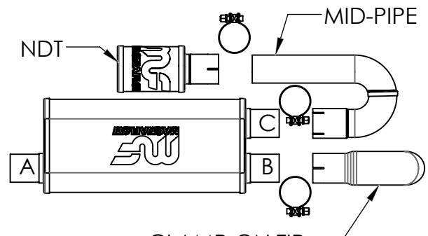
CLAMP-ON TIP
