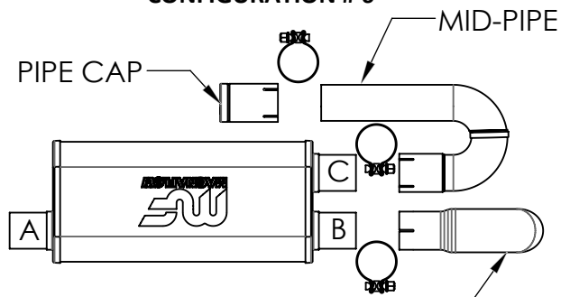
CLAMP-ON TIP
