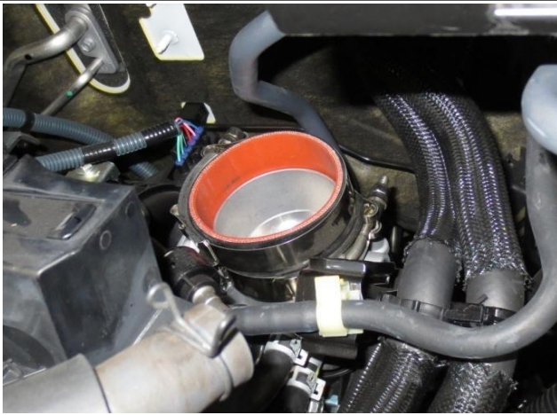
4. Install the 3" coupler along with the T-bolt clamps onto the throttle body.
