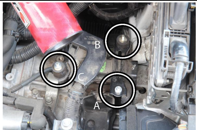
7. (A) Thread in and secure the provided M6 x 20mm bolt through the bottom of the bracket and insert the 5mm spacer. (B) Insert the provided 1/2" vibration mount onto the factory air box mount. (C) Insert the provided 1" vibration mount and insert the 5mm spacer.
