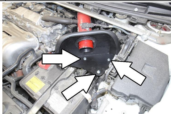
9. Insert the heat shield into the vehicle and secure the heat shield using the provided M6 nuts and washers.
